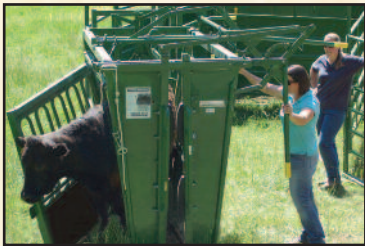
XL Manual Chute with Right Exit Order No. 002-10052 (Shown with optional Neck Extender Order number. 002-20000)
